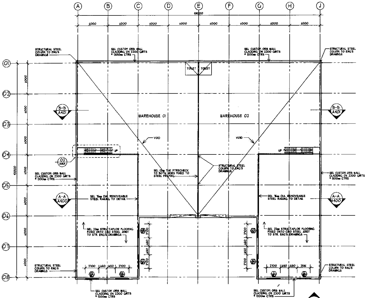
PROPOSED MEZZANINE FLOOR PLAN SCALE 1 : 200
